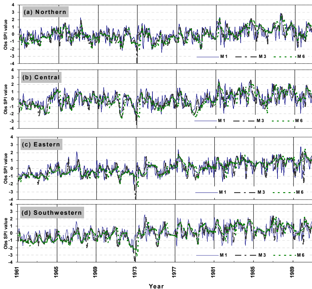
Figure 2. The SPI values calculated from regional rainfall data for 1 month (M1), 3 month (M3) and 6 month (M6) length at (a) northern (b) central (c) eastern and (d) southwestern sub-regions of Bangladesh during 1961 to 1990.
